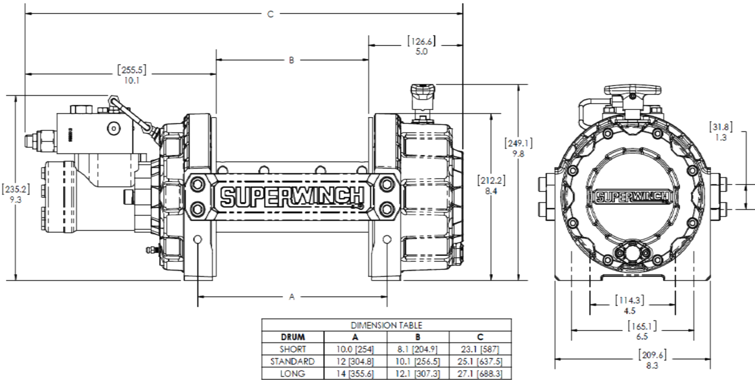
OVERALL DIMENSIONS Units: IN [mm]
