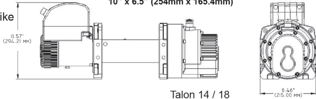
Mounting Bolt Pattern: 10" x 4.5" (254mm x 114.3mm) & 10" x 6.5" (254mm x 165.4mm)
